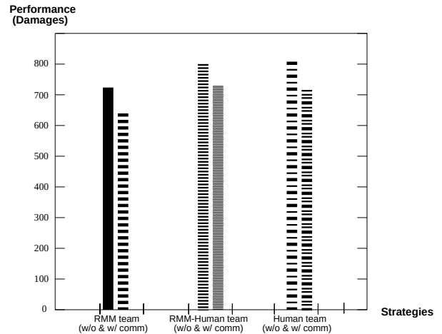
Figure 2: The performance of RMM, RMM-Human, and Human teams in anti-air defense, without and with communication, respectively.
