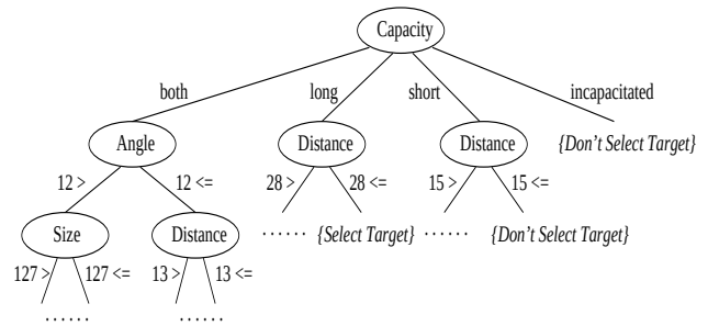
Figure 6: The decision tree obtained by C4.5.
